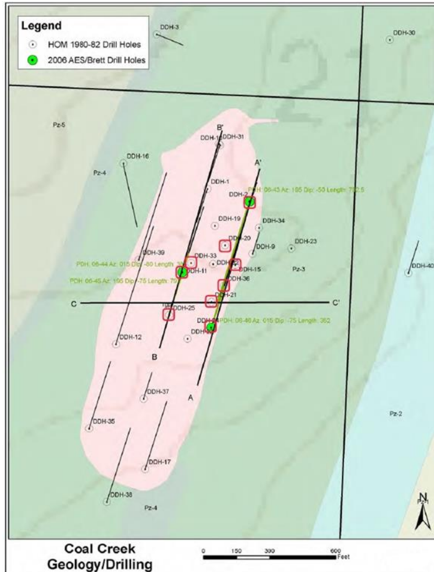
Figure 1. Chulitna Project – Coal Creek Historic Drill Hole Location Map (scanned drill holes highlighted in red)
